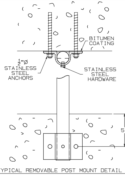
TYPICAL REMOVABLE POST MOUNT DETAIL
