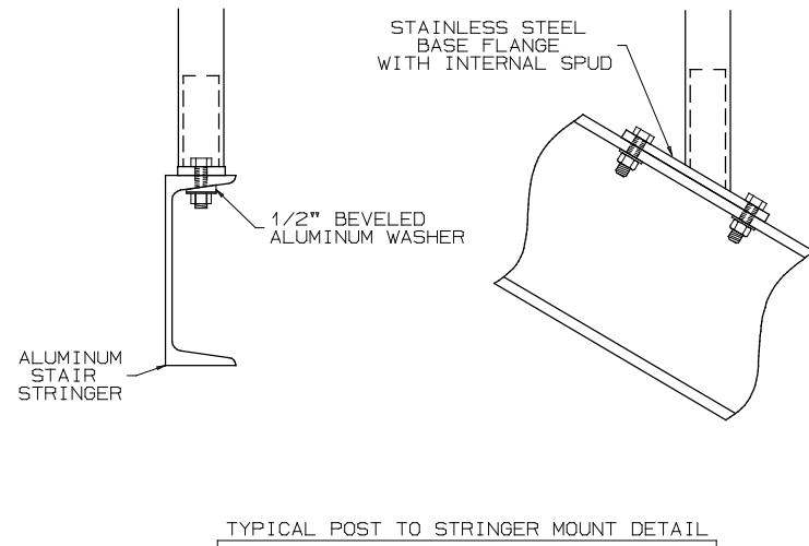
TYPICAL POST TO STRINGER MOUNT DETAIL
