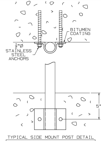
TYPICAL SIDE MOUNT POST DETAIL
