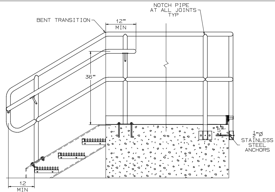
TYPICAL GUARDRAIL AT METAL STAIR
