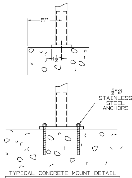
TYPICAL CONCRETE MOUNT DETAIL
