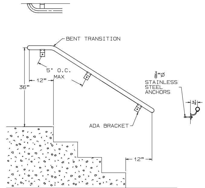
TYPICAL WALL MOUNTED HANDRAIL
