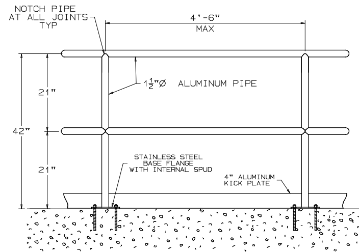
TYPICAL GUARDRAIL
